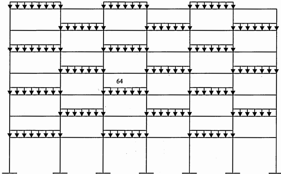
Figure 7.1. Case 1: Live load pattern for maximum span moments in beam
