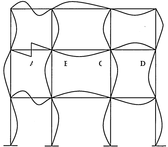
Figure 2.1a. Influence line for positive shear at mid-span of AB
