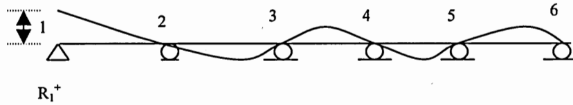
Figure 1.1a. Influence Line for positive reaction at support 1
