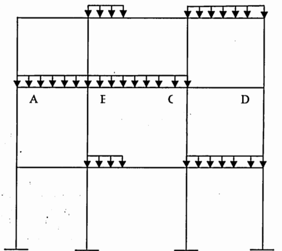
Figure 2.3b. Load Pattern for maximum negative moment at B
