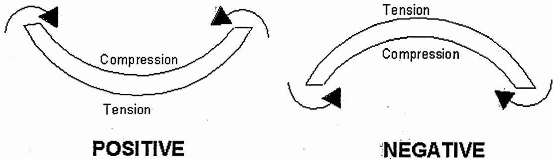
Figure 1.3. Sign convention for positive and negative bending moment
