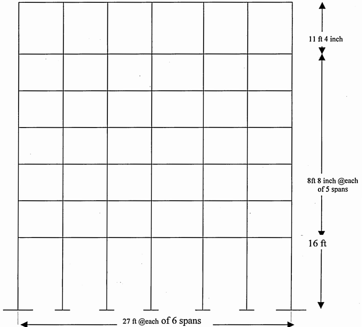
Figure 6.2. Portal Frame in consideration (six bays & seven stories)
