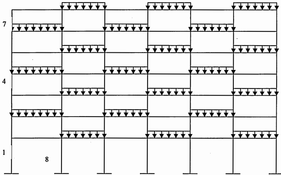
Figure 7.5. Case 3: Live load pattern C for maximum/minimum end moment in a column
