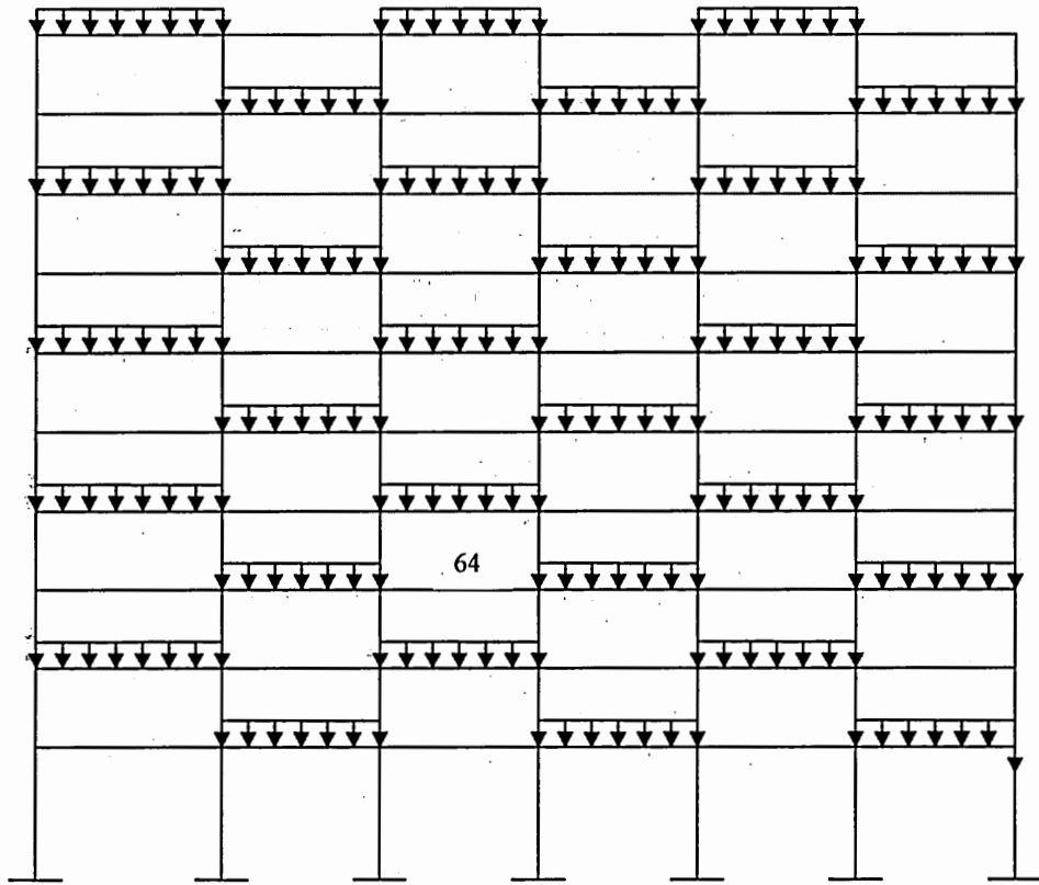
Figure 9.2. Case 2: Live load pattern for minimum span moment in beam – ten-floor frame
