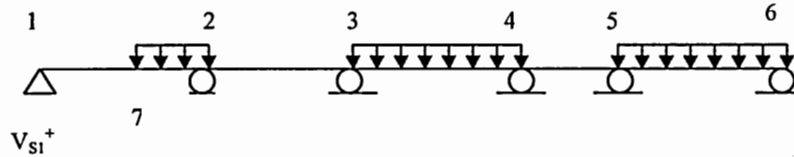
Figure 1.7b. Load pattern for maximum positive shear at 7
