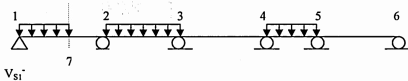
Figure 1.8b. Load pattern for maximum negative shear at 7
