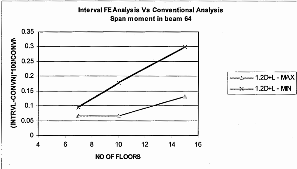
Figure 12b. Maximum and Minimum Span Moment in Beam 64 - Percentage deviation Vs number of floor for load combination 1.2 D + L
