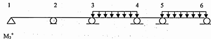
Figure 1.4b. Load pattern for maximum positive moment at support 2
