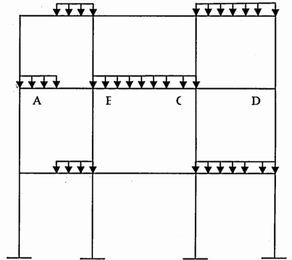
Figure 2.2b. Load Pattern for maximum negative shear at mid-span of AB
