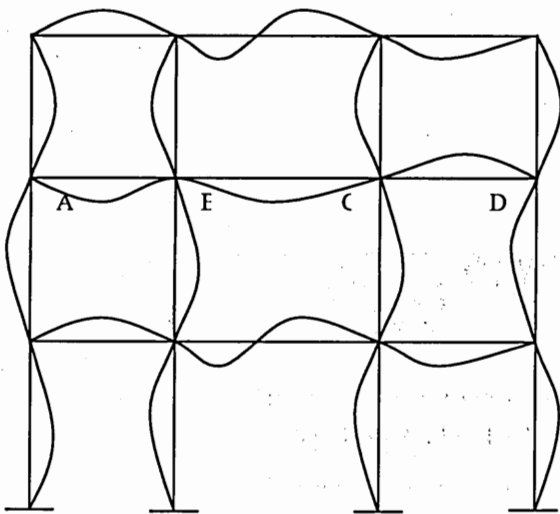
Figure 2.3a. Influence line for negative moment at B
