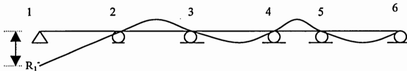
Figure 1.2a. Influence Line for negative reaction at support 1
