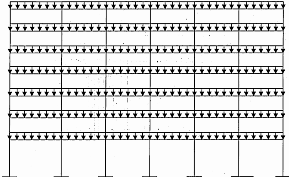
Figure 3.1. Dead Load Presence on a Portal Frame
