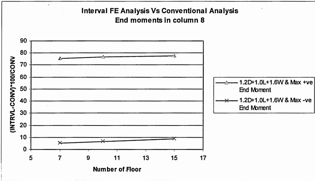
Figure 13b. Bounds on End Moment in Column 8- Percentage Vs number of floor for load combination 1.2D+1.0L+1.6W
