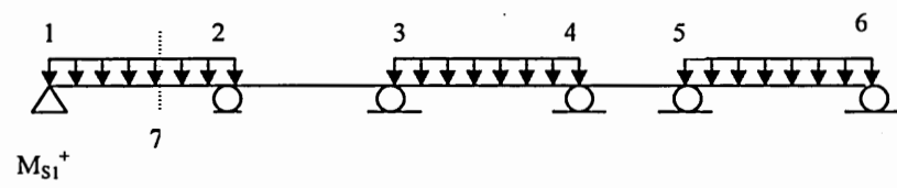
Figure 1.9b. Load pattern for maximum positive moment at 7
