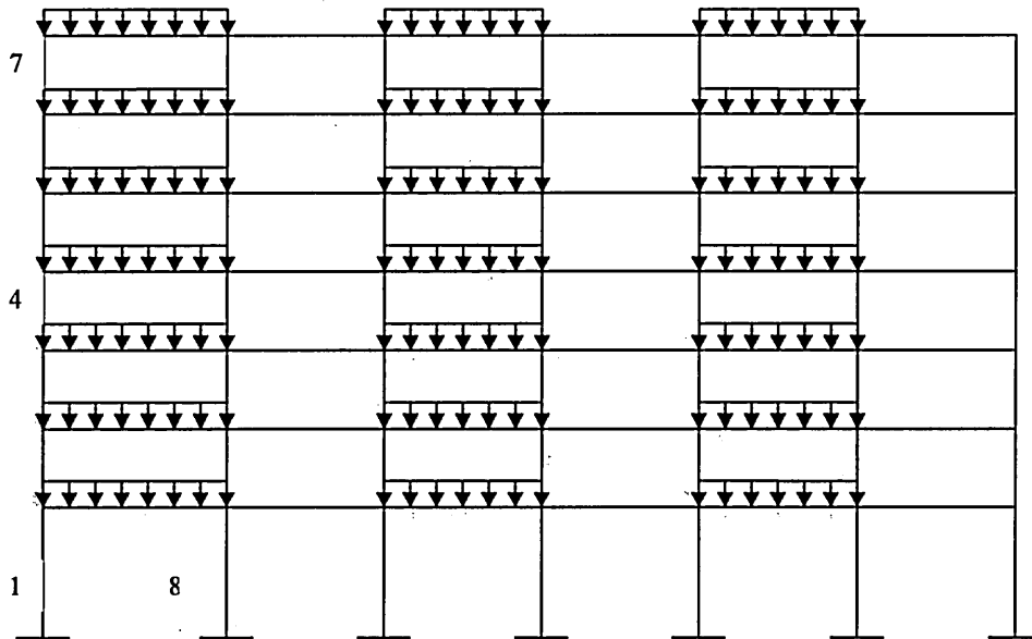
Figure 7.3. Case 3: Live load pattern A for maximum/minimum end moment in a column
