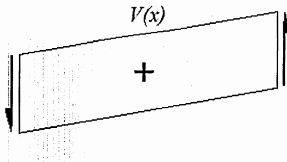
Figure 1.6. Sign convention for positive shear
