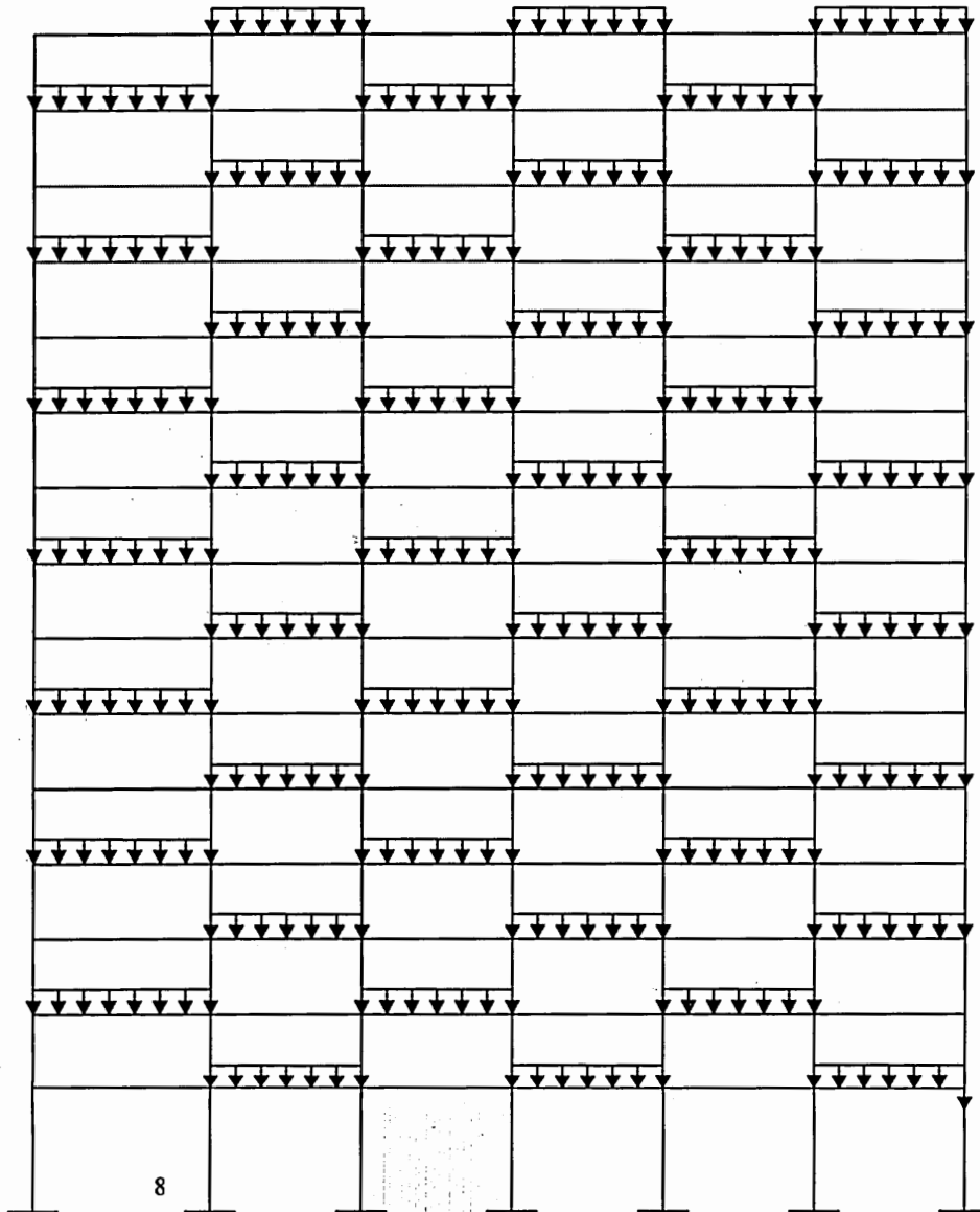
Figure 11.5. Case 3: Live load pattern C for maximum/minimum end moment in column– fifteen-floor frame
