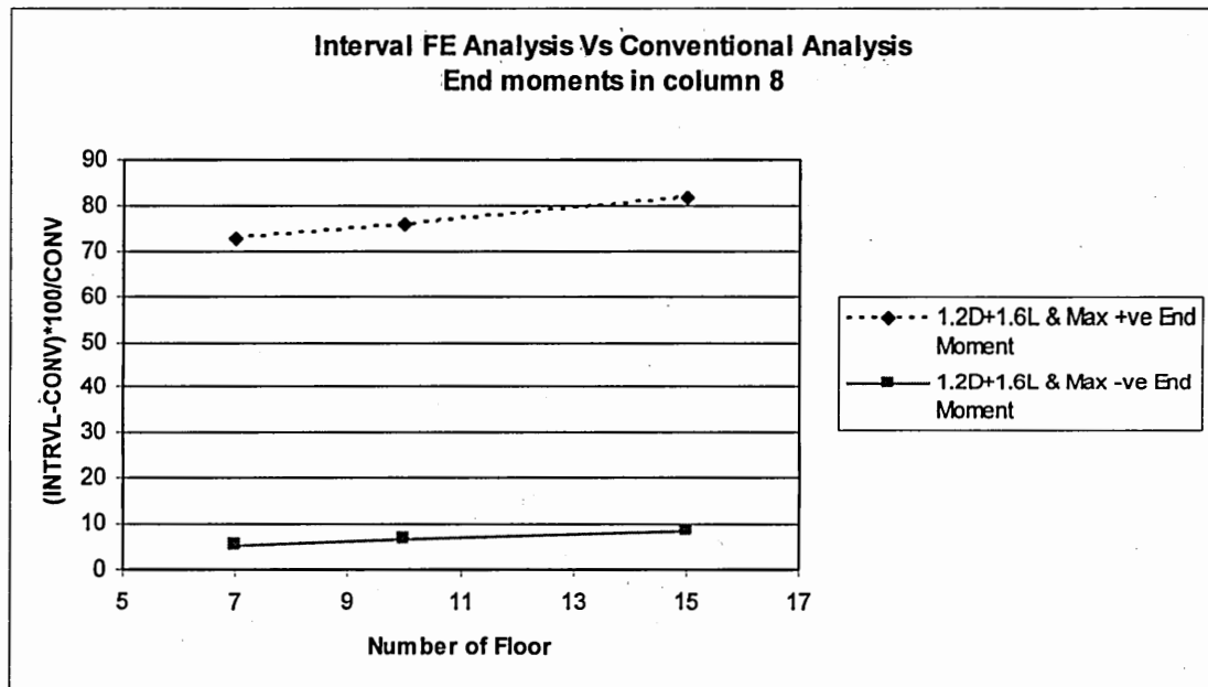
Figure 13a. Bounds on End Moment in Column 8- Percentage Deviation Vs number of floor for load combination 1.2D+1.6L
