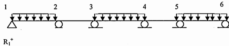
Figure 1.1b. Load pattern for maximum positive reaction at support 1
