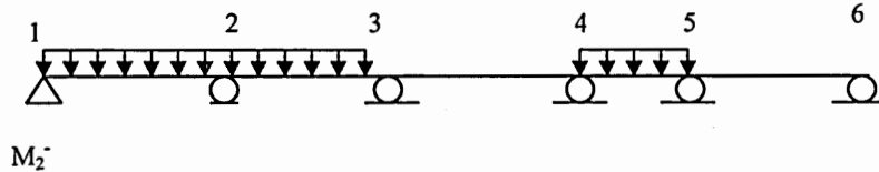
Figure 1.5b. Load pattern for maximum negative moment at support 2
