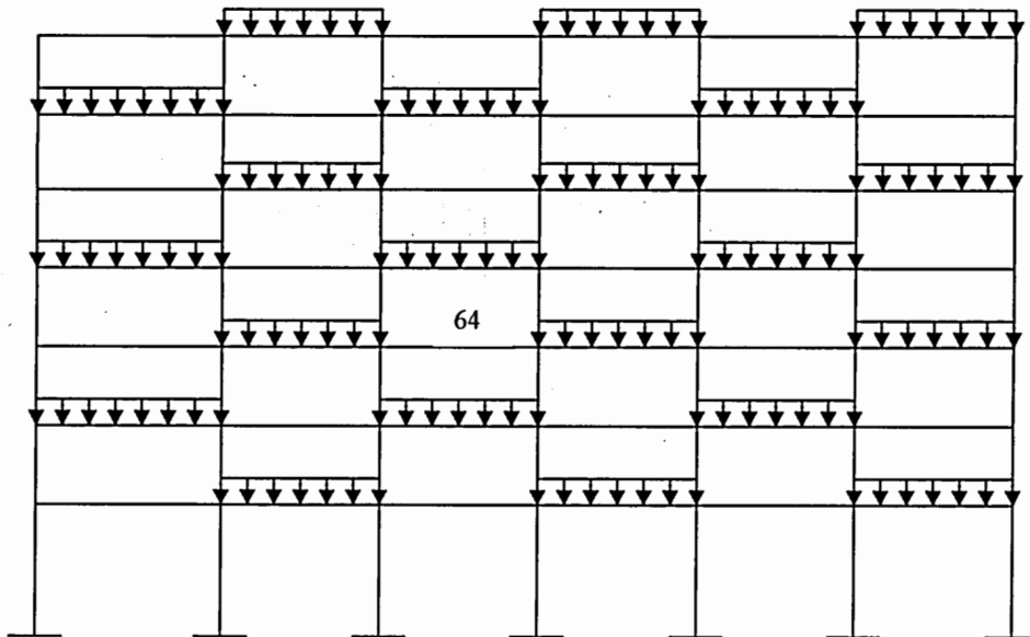
Figure 7.2. Case 2: Live load pattern for minimum span moment in beam
