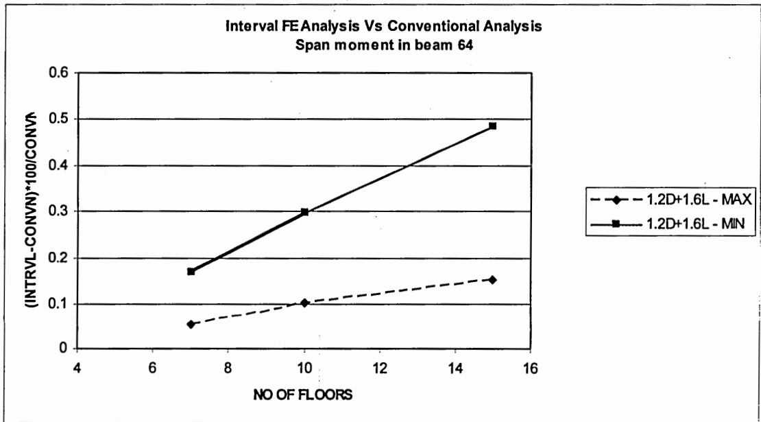
Figure 12a. Maximum and Minimum Span Moment in Beam 64 - Percentage deviation Vs number of floor for load combination 1.2 D + 1.6 L
