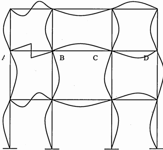
Figure 2.2a. Influence line for negative shear at mid-span of AB
