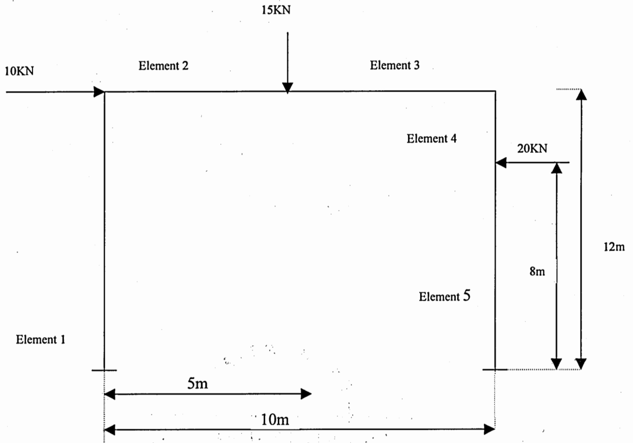
Figure 5. Finite Element consisting five nodes and six-frame element
