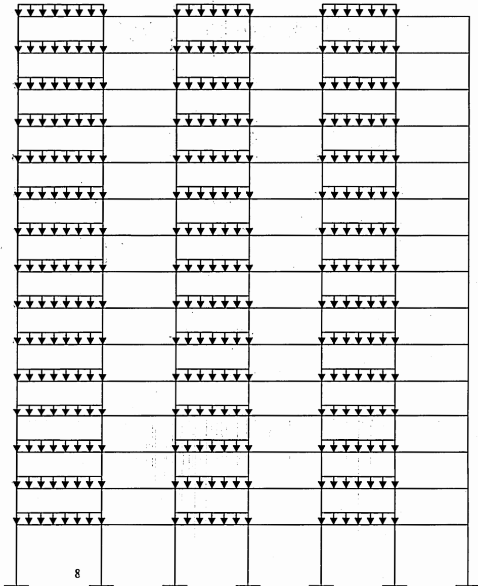
Figure 11.3. Case 3: Live load pattern A for maximum/minimum end moment in column- fifteen-floor frame
