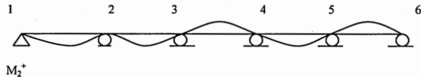
Figure 1.4a. Influence Line for positive moment at support 2
