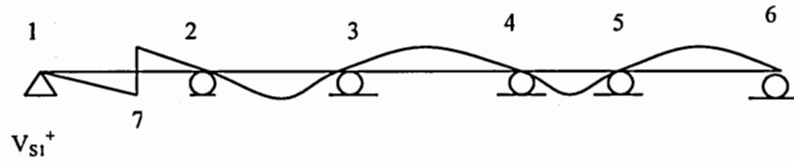
Figure 1.7a. Influence line for positive shear at 7
