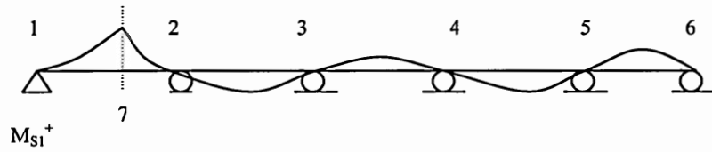
Figure 1.9a. Influence line for positive moment at 7
