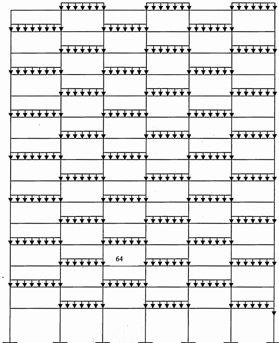
Figure 11.2. Case 2: Live load pattern for minimum span moment in beam element – fifteen floors frame
