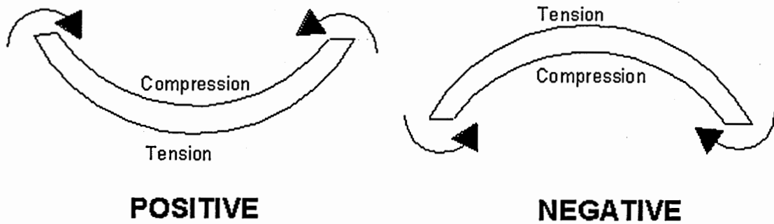
Figure 7.0. Sign convention for positive and negative bending moment
