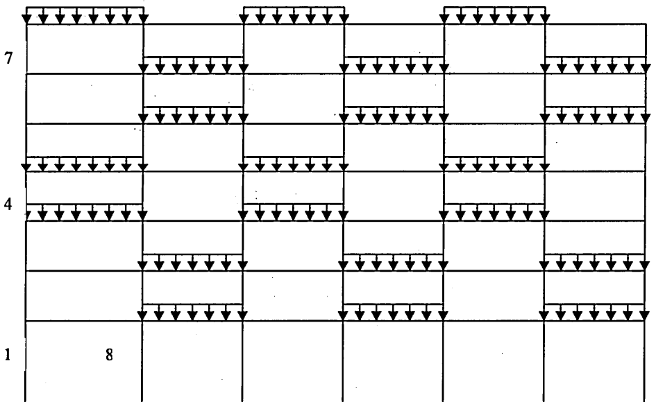
Figure 7.4. Case 3: Live load pattern B for maximum/minimum end moment in a column
