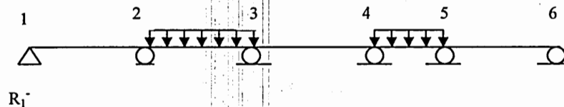
Figure 1.2b. Load pattern for maximum negative reaction at support 1
