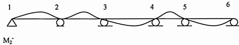
Figure 1.5a. Influence line for negative moment at support 2
