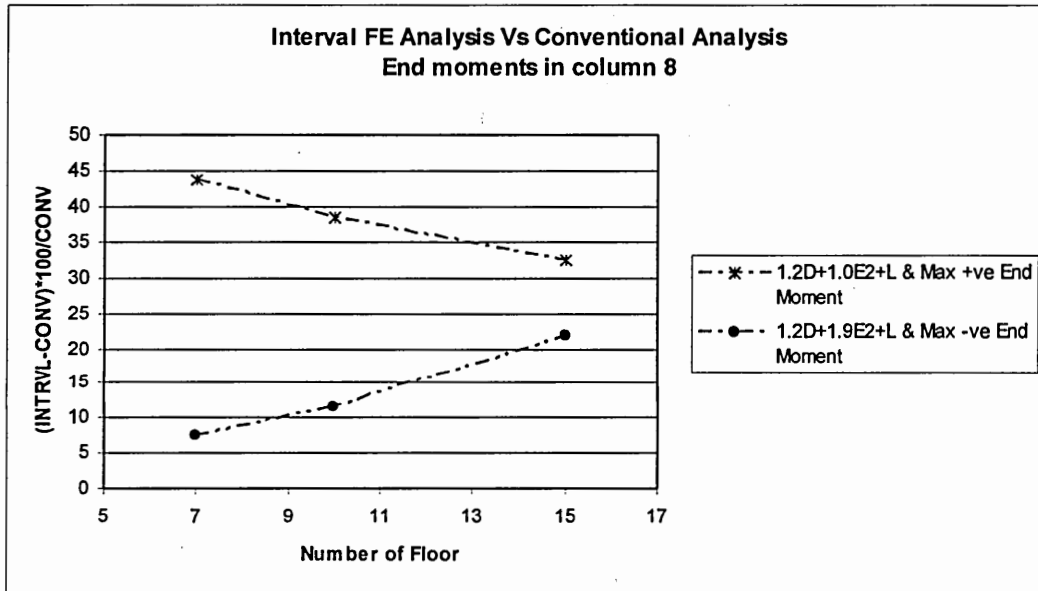
Figure 13c. Bounds on End Moment in Column 8- Percentage Deviation Vs number of floor for load combination 1.2D+1.0E2+L
