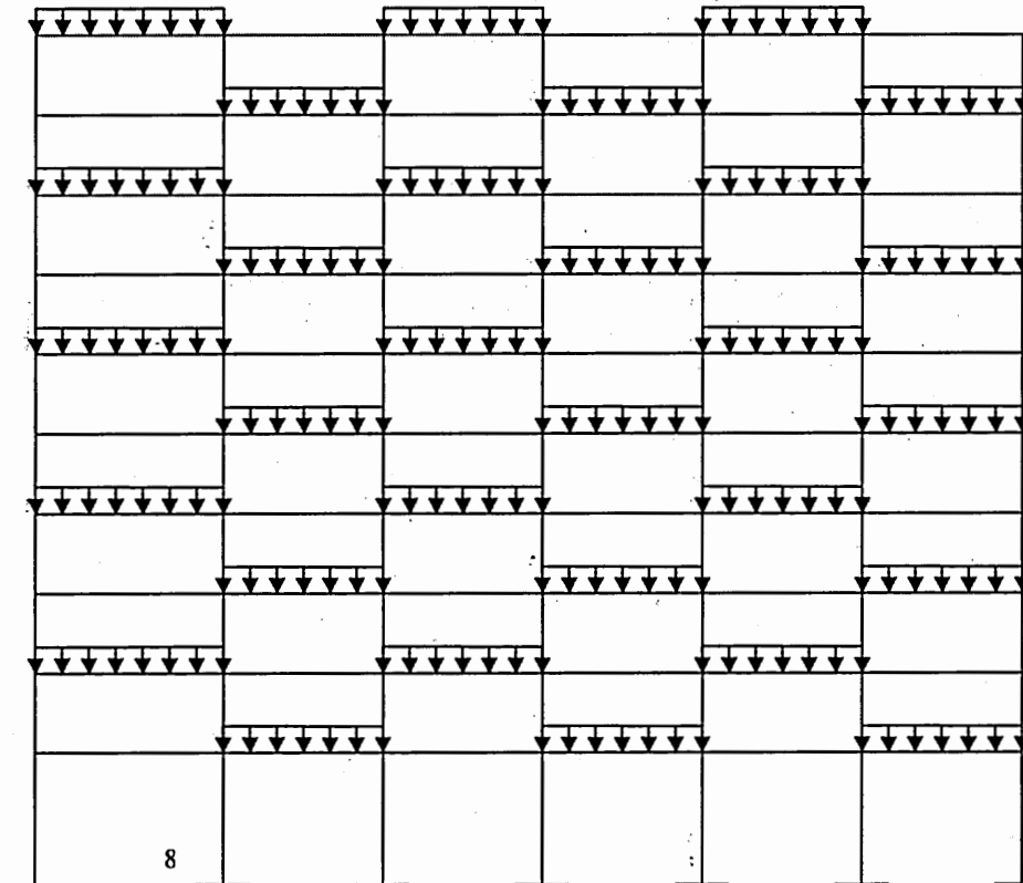
Figure 9.5. Case 3: Live load pattern C for end moment at the end of column— ten floors frame
