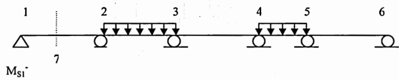
Figure 1.10a. Influence line for negative moment at 7
