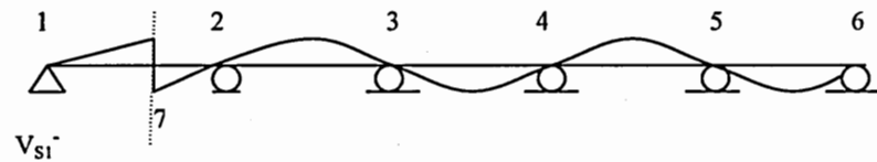
Figure 1.8a. Influence line for negative shear at 7
