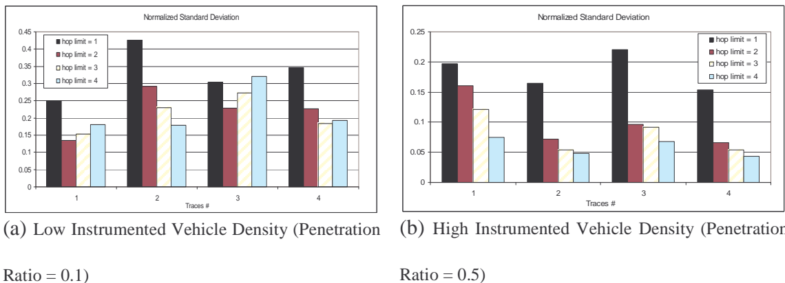
Figure 31: Normalized standard deviation of the number of instrumented vehicles connected to WLAN over its mean for a time scale of 1 second for different hop limits
