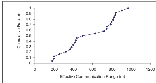
Figure 47: The cumulative distribution of effective communication ranges between 2 vehicles moving in opposite directions
