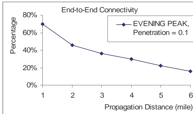
Figure 16: Evening peak end-to-end connectivity for fleet penetration ratio of 0.1
